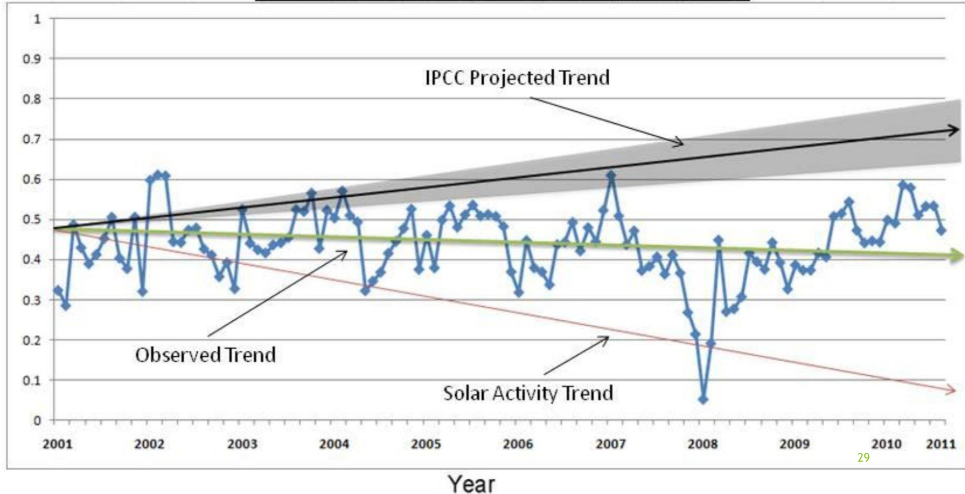
Observed & Projected Temperature Trends
